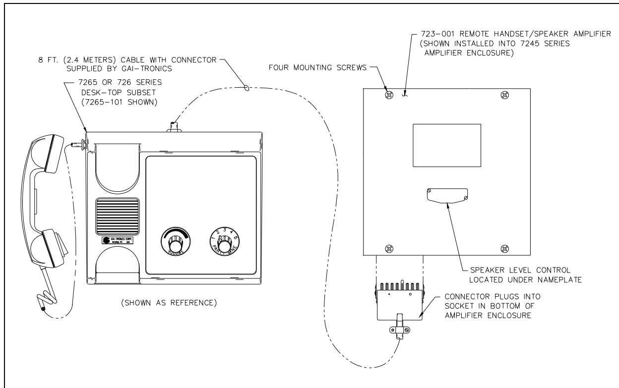
Figure 1. Installation of the 723-001 Remote Handset/Speaker Amplifier
